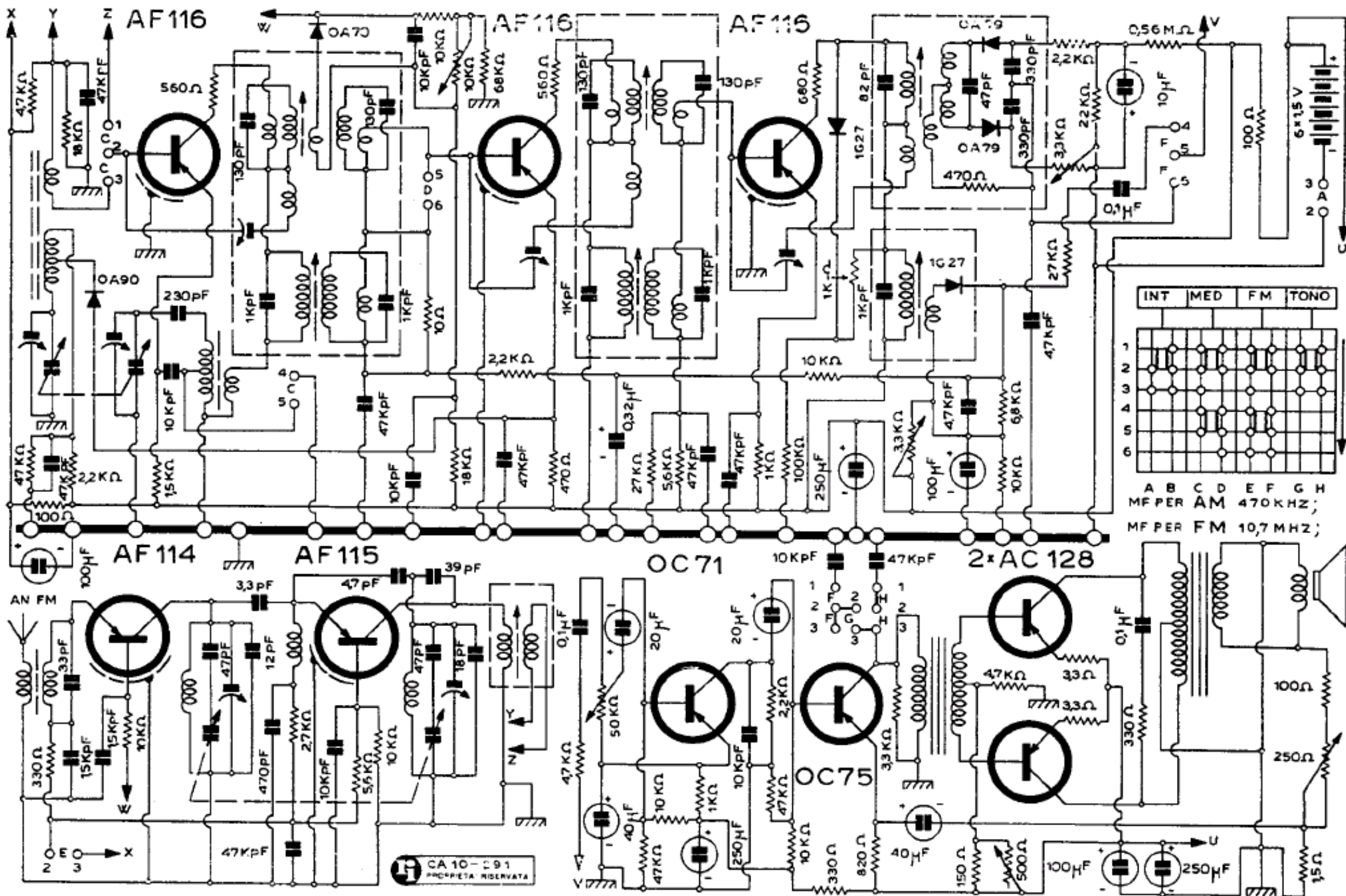
FIMI - Mod. Phonola RT 9127 "Strato Cruiser,"
